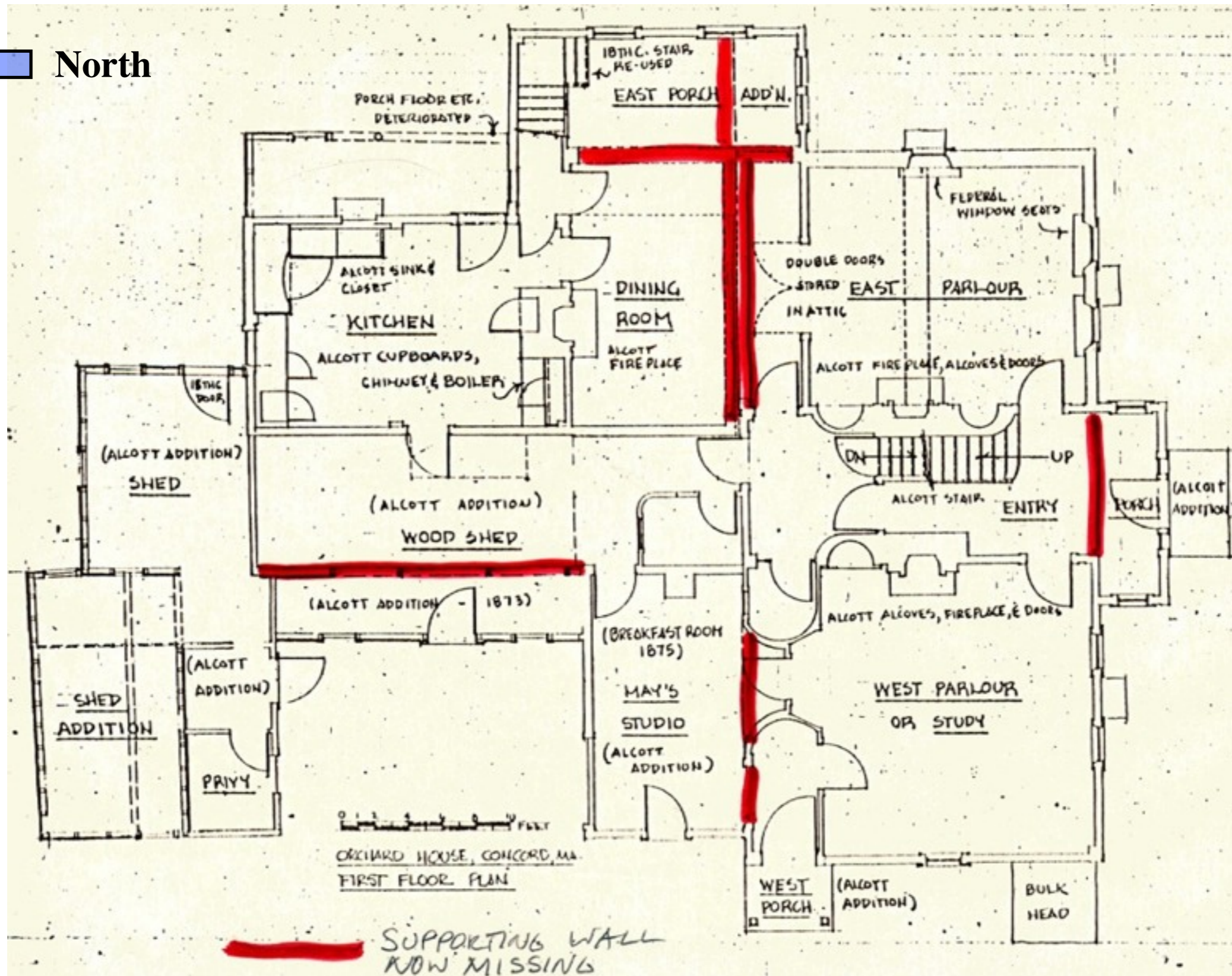
Figure E-3. Orchard House, First Floor Plan, 1980, drawing by F.C. Detwiler, Architectural Historian. DWT 9/81
